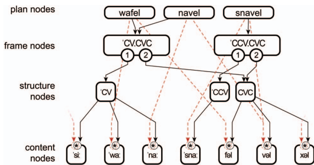
Figure 1. An instance of the EPONA model containing the nodes necessary to produce the Dutch disyllabic words wafel ['wa:fəl] “waffle,” navel ['na:vəl] “navel” and snavel ['sna:vəl] “beak.” The segmental route is shown with red dashed connections. At the top level, there is a unique plan node for each word. Frame nodes are shared between words with the same metrical structure ( wafel and navel both have a 'CV.CVC structure, so are connected to the same frame node). Each frame node has multiple output ports (here numbered 1 and 2), one associated with each child element of the sequence. Each port is connected to a structure node. In turn, each structure node is connected to all content nodes representing syllables with the relevant metrical structure. Structure nodes and content nodes are also shared between words. Multiplication in the content nodes (represented by asterisks) ensures that only syllables receiving input from both routes become active. See the online article for the color version of this figure.
